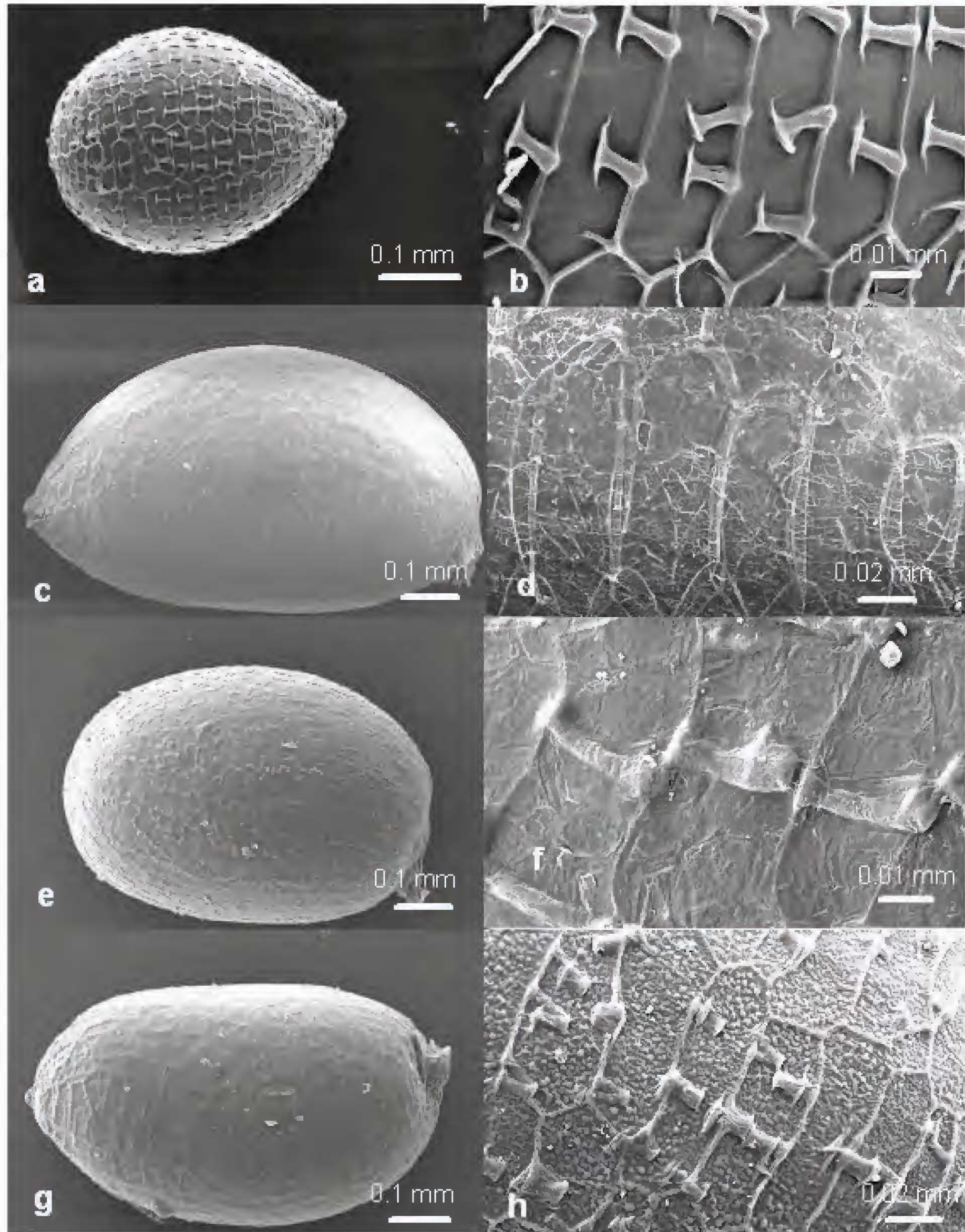
Fig. 3. Seed and seed surface: Eriocaulon carpentariae a, b ; E. carsonii subsp. carsonii c, d ; E. carsonii subsp. euloense e, f ; E. carsonii subsp. orientale g, h . Material used: a-b from Beaughlehole 54794 ; c-d from Peery Lake 4, 5 ; e-f from Bundoona Stn 1 and 3 ; g-h from Davies 95 .
